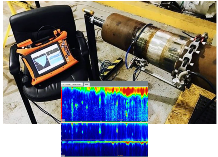
DMA Probe L-Wave, Iconel 625 - Single V, 50mm thick with 12.4mm stainless cladding
